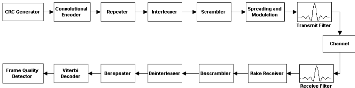
IS-95A Forward Channel Diagram
