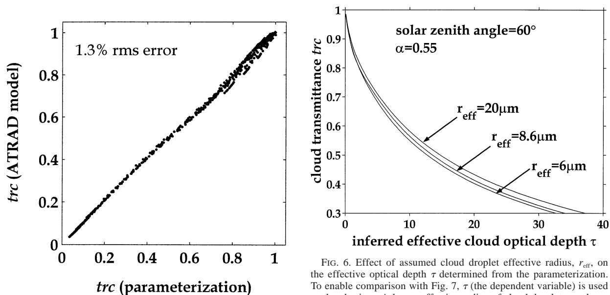
FIG. 5. Comparison of transmittance obtained from the radiative transfer model to that obtained from the parameterization, using a synthetic dataset, an rms error of 1.3% is shown.
