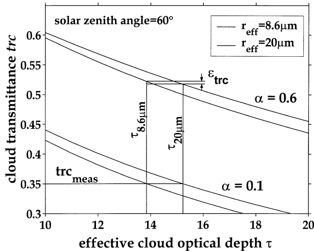
FIG. 7. Example of the error in derivation of cloud radiative properties due to lack of knowledge of the drop-size distribution. The cloud was observed over a surface of albedo 0.1, and the measured transmittance of solar radiation ( trc ) was 0.35. If we assume r_{eff} = 8.6 \mu m we obtain \tau = 13.8 . We estimate using the parameterization [Eq. (1)] that if this cloud were placed over a surface of albedo 0.6, it would have trc = 0.528 . If we instead had larger drops ( r_{eff} = 20 \mu m ), we infer \tau = 15.2 , and estimate that if this cloud were placed over the high-albedo surface it would have trc = 0.512 , very close to that estimated using the smaller drops. Lack of knowledge of r_{eff} in this case causes errors of 10%–15% in the intermediate quantity \tau but only 2% in the prediction of solar transmittance in a different environment.
