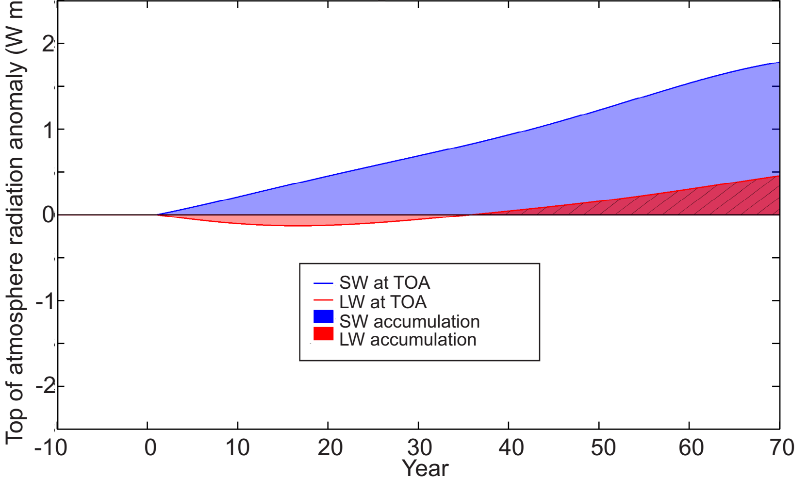
CMIP3 ensemble average response to 1% per year \text{CO}_2 increase to doubling
