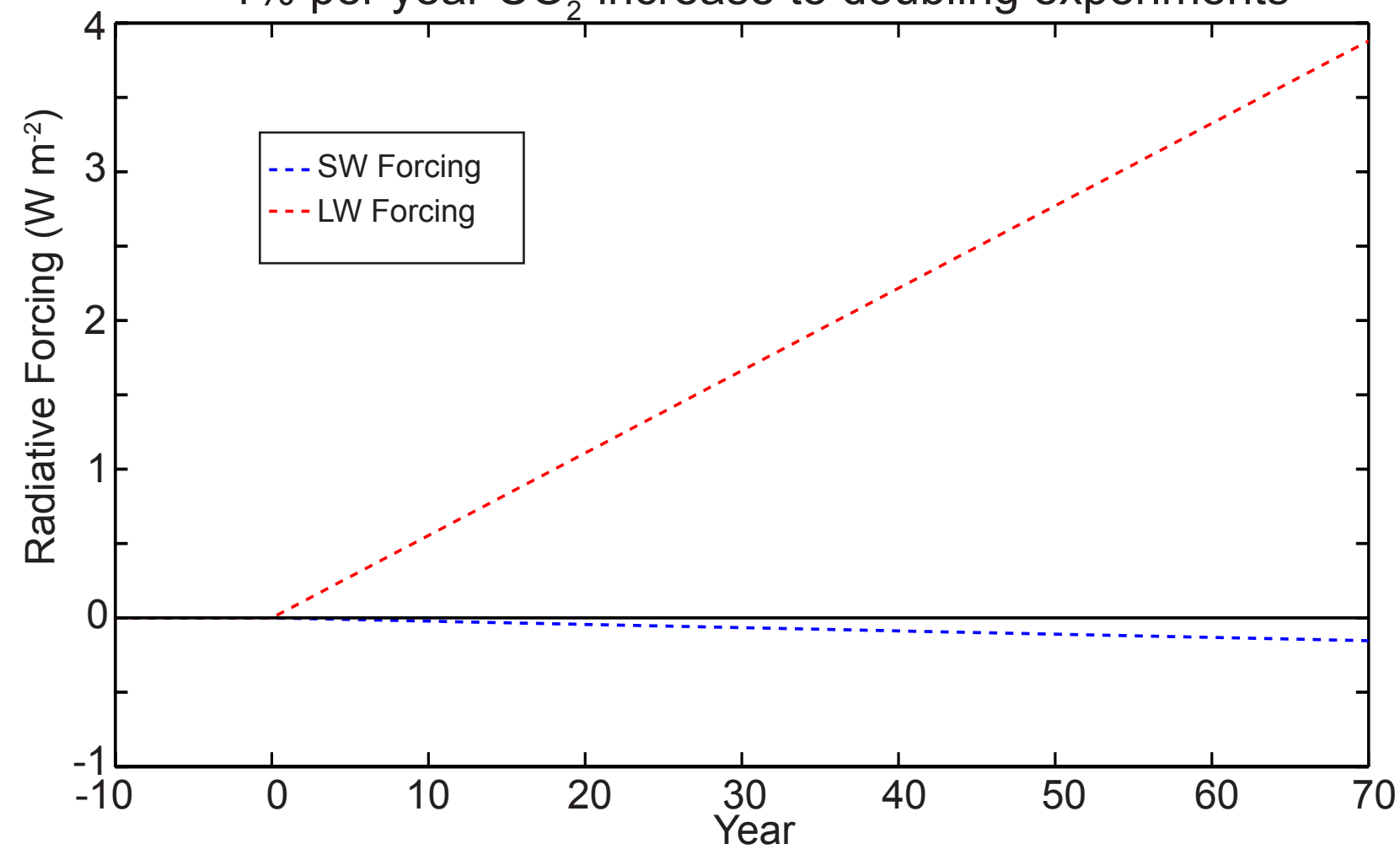
Radiative forcing 1% per year \text{CO}_2 increase to doubling experiments
