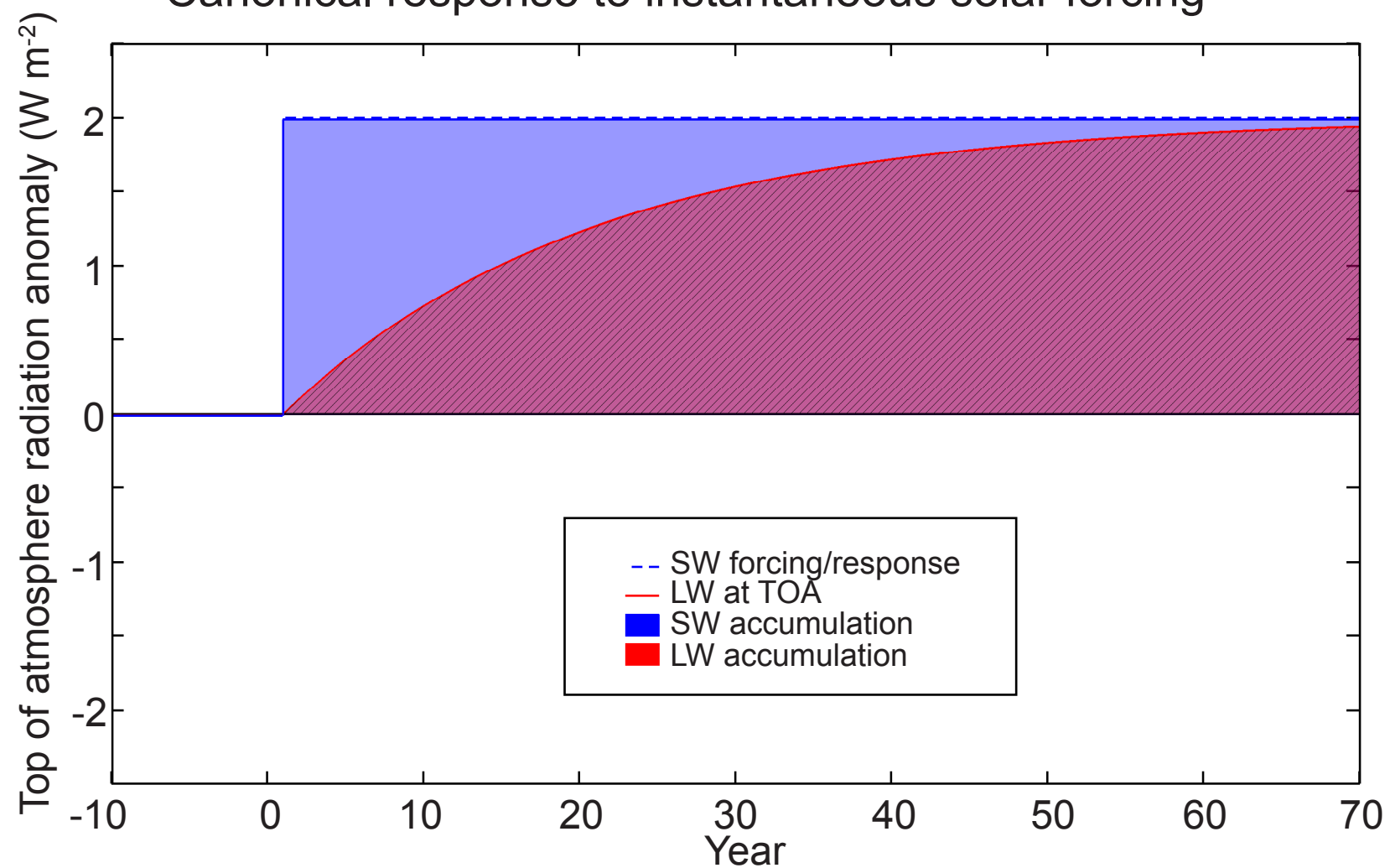
Canonical response to instantaneous solar forcing
