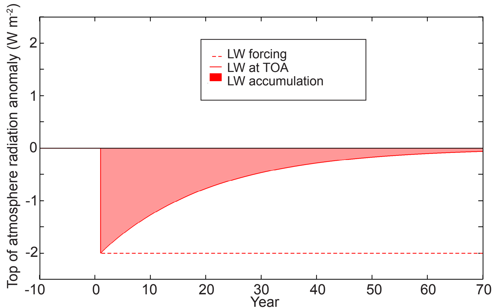
Canonical response to instantaneous greenhouse forcing
