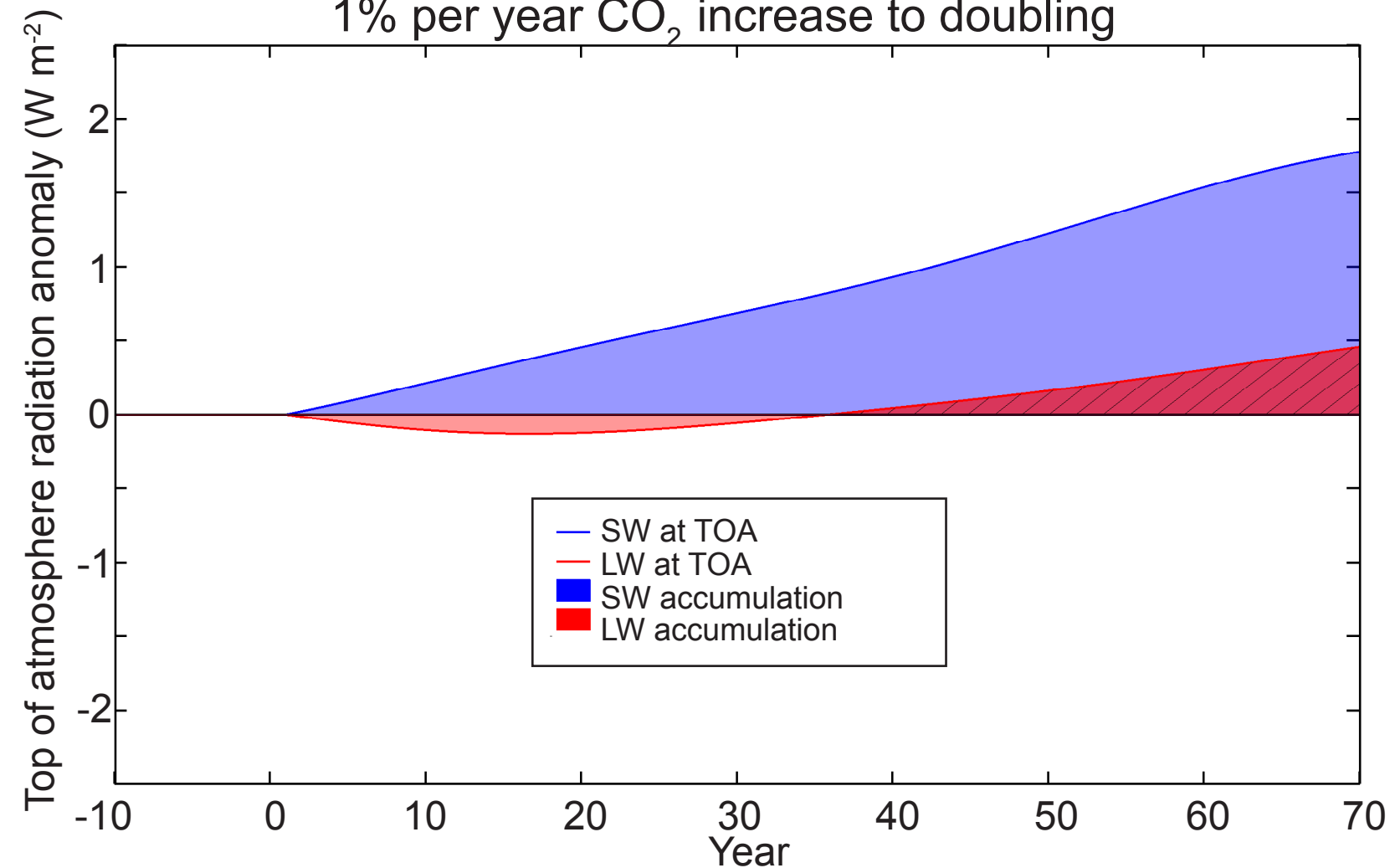
Radiative forcing 1% per year \text{CO}_2 increase to doubling experiments
