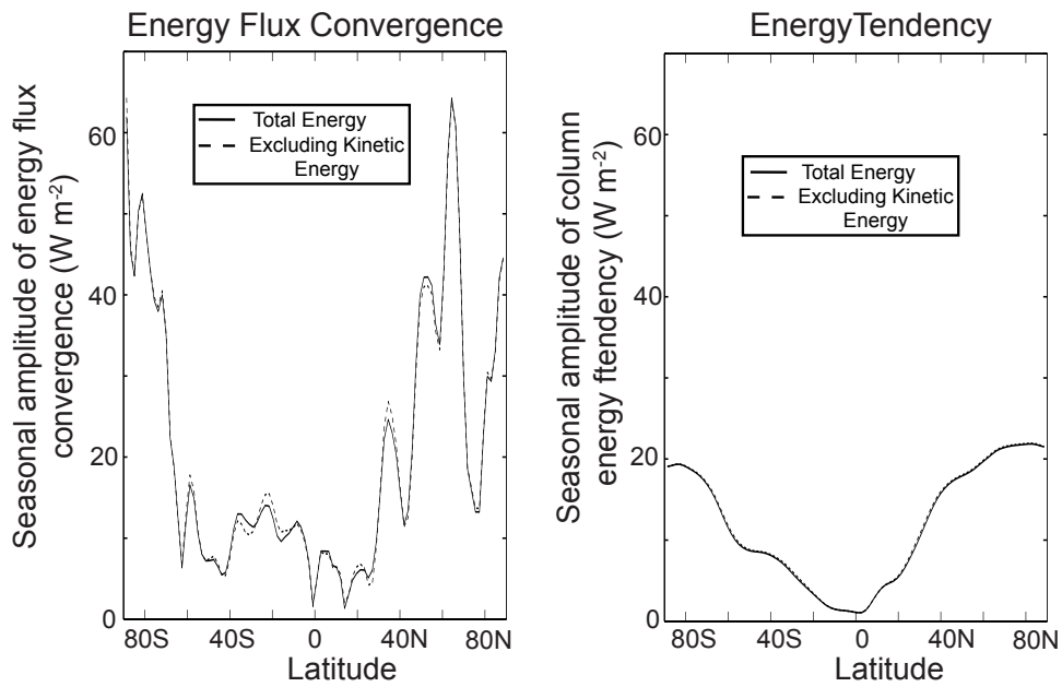
Figure 8: The seasonal amplitude (the amplitude of the annual Fourier harmonic) of the horizontal energy flux convergence (left panel) and the energy tendency. The solid line is the total energy and the dashed line is the total energy minus the kinetic energy. All calculations were done from Trenberth and Stepaniak's (2003) data.
