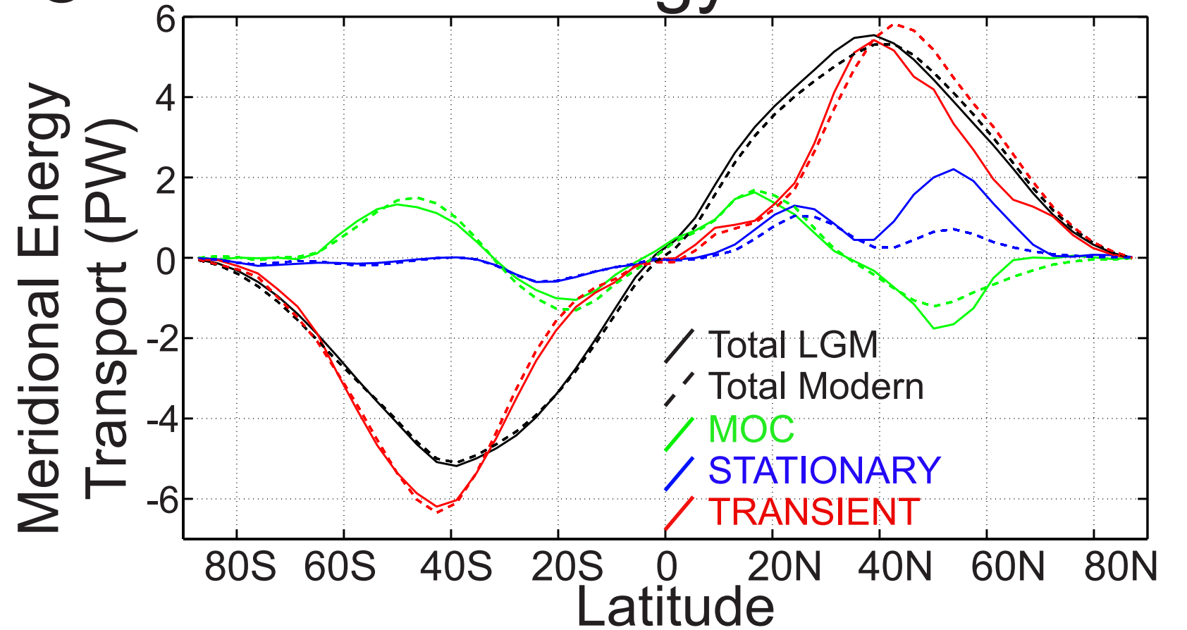
C Meridional Energy Flux Partition
