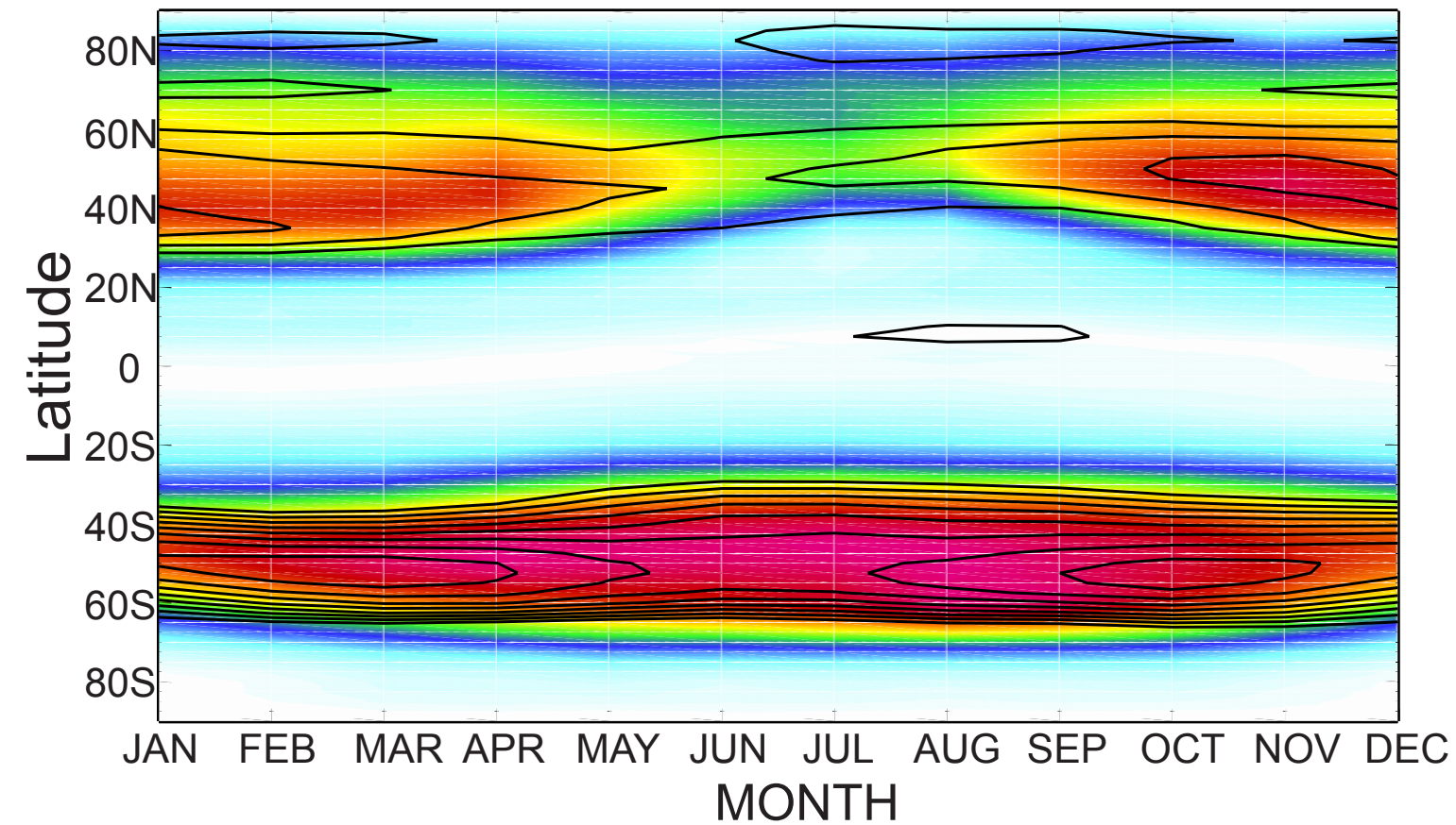
A Observed seasonal cycle of surface zonal winds (contours) and transient eddy energy flux (colors)
