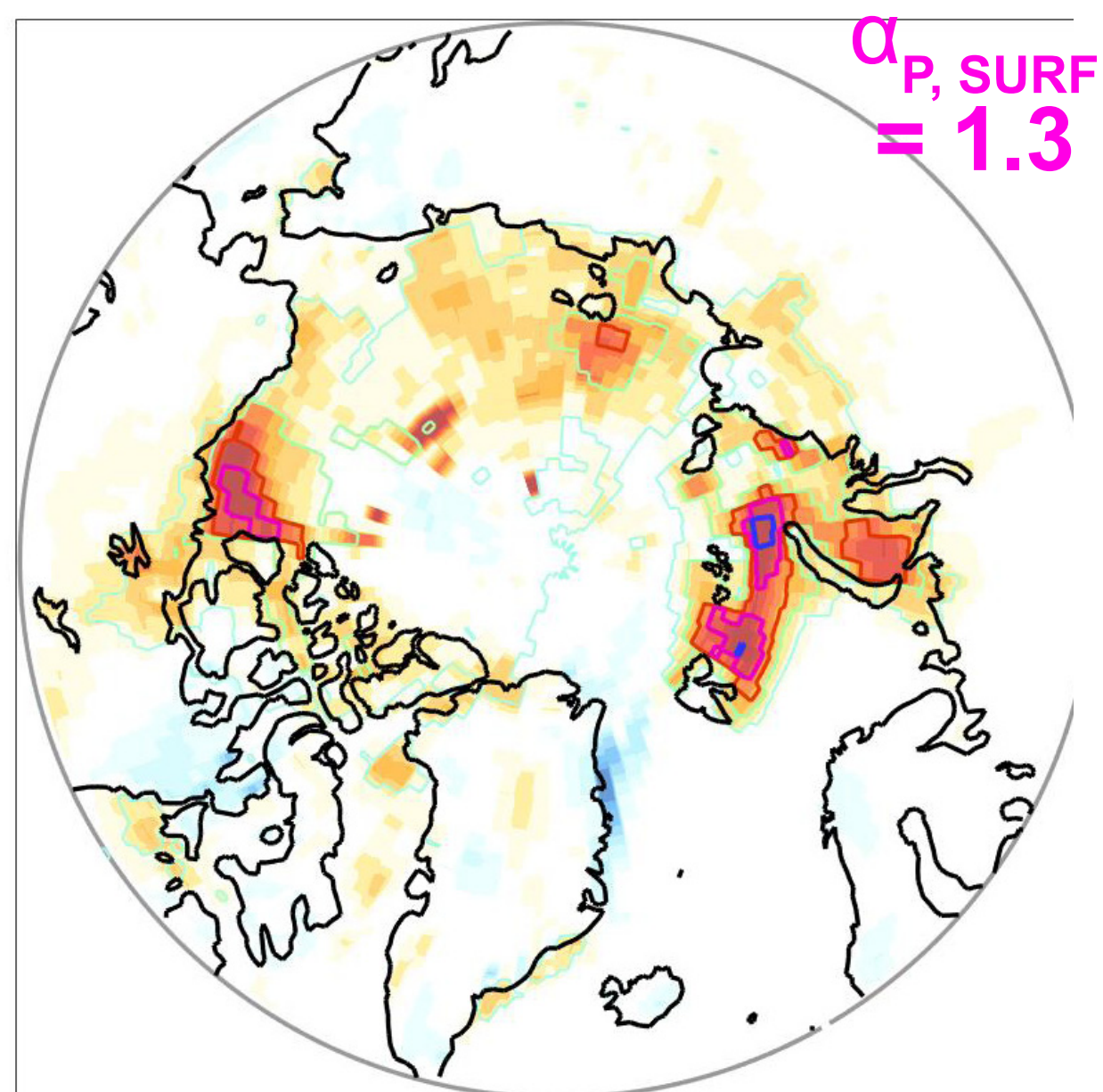
Surface Albedo Anomaly Times Insolation ( \text{W m}^{-2} )
