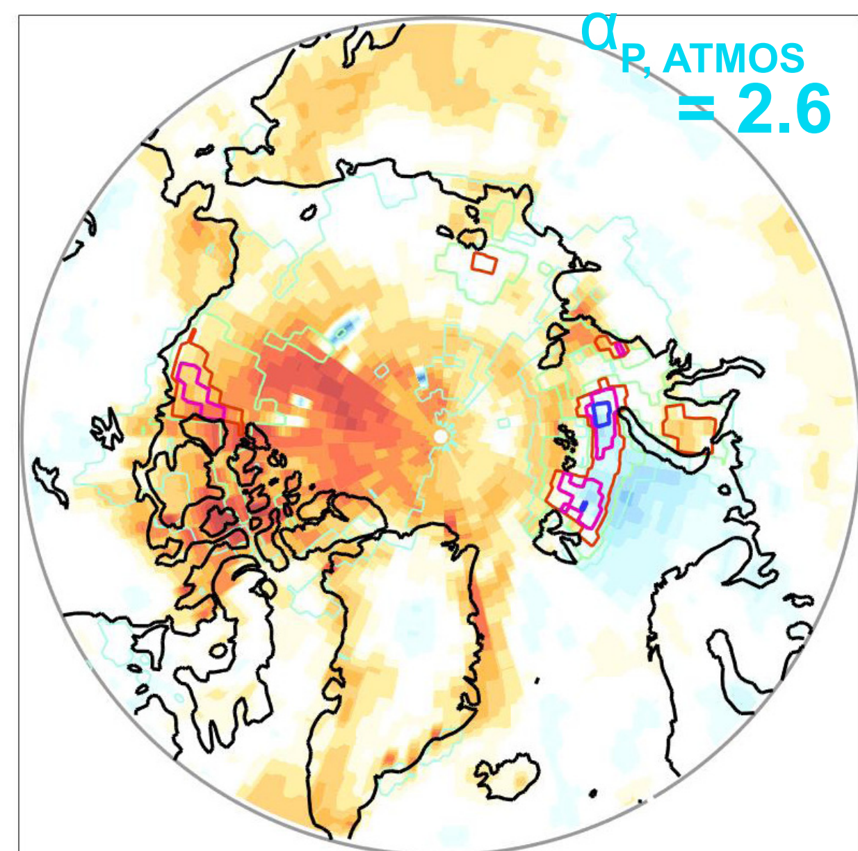
TOA reflected solar ( \text{W m}^{-2} )
