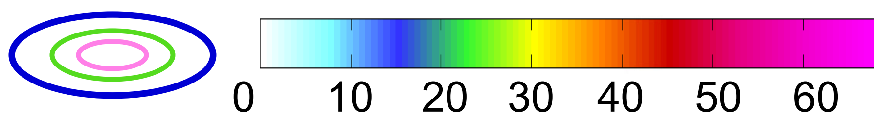
Surface Albedo Anomaly Times Insolation ( \text{W m}^{-2} )
