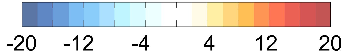
TOA reflected solar ( \text{W m}^{-2} )
