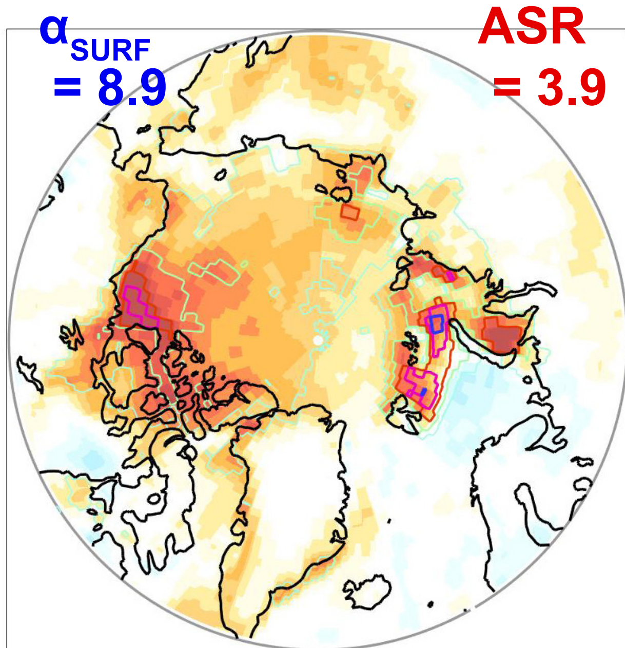
Surface Albedo Anomaly Times Insolation ( \text{W m}^{-2} )
