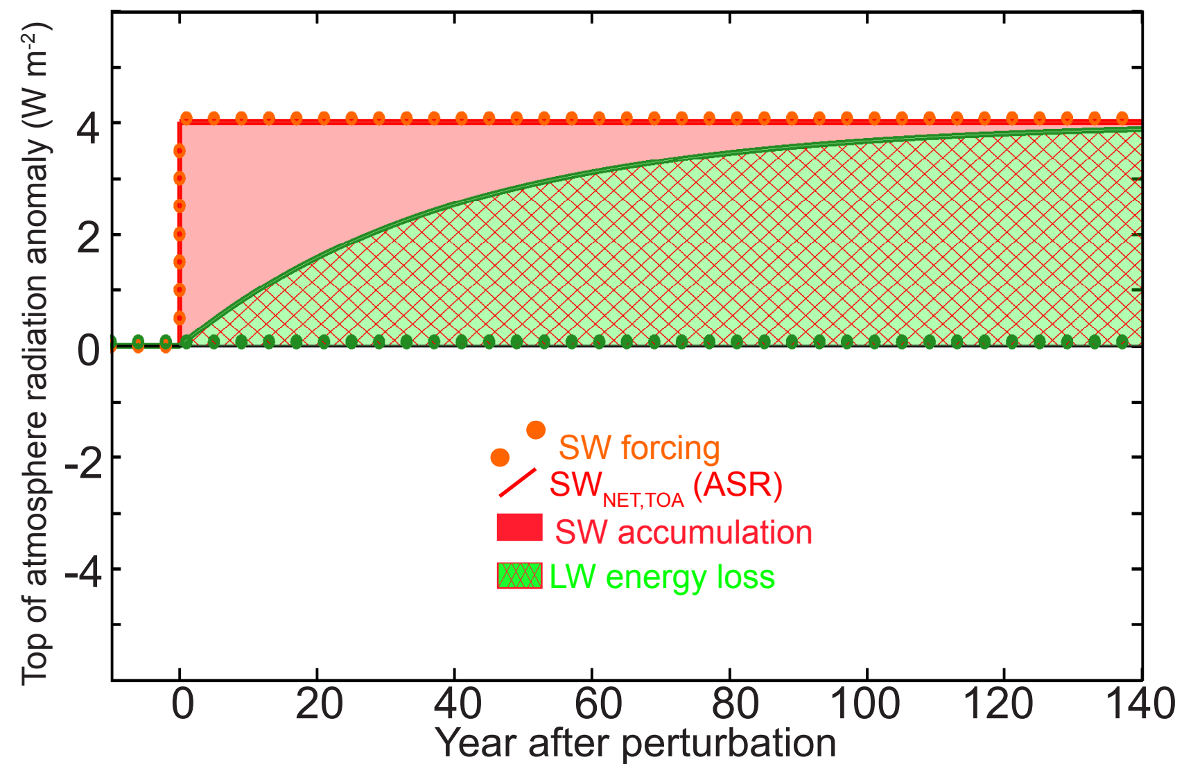
B Canonical response to instantaneous solar forcing
