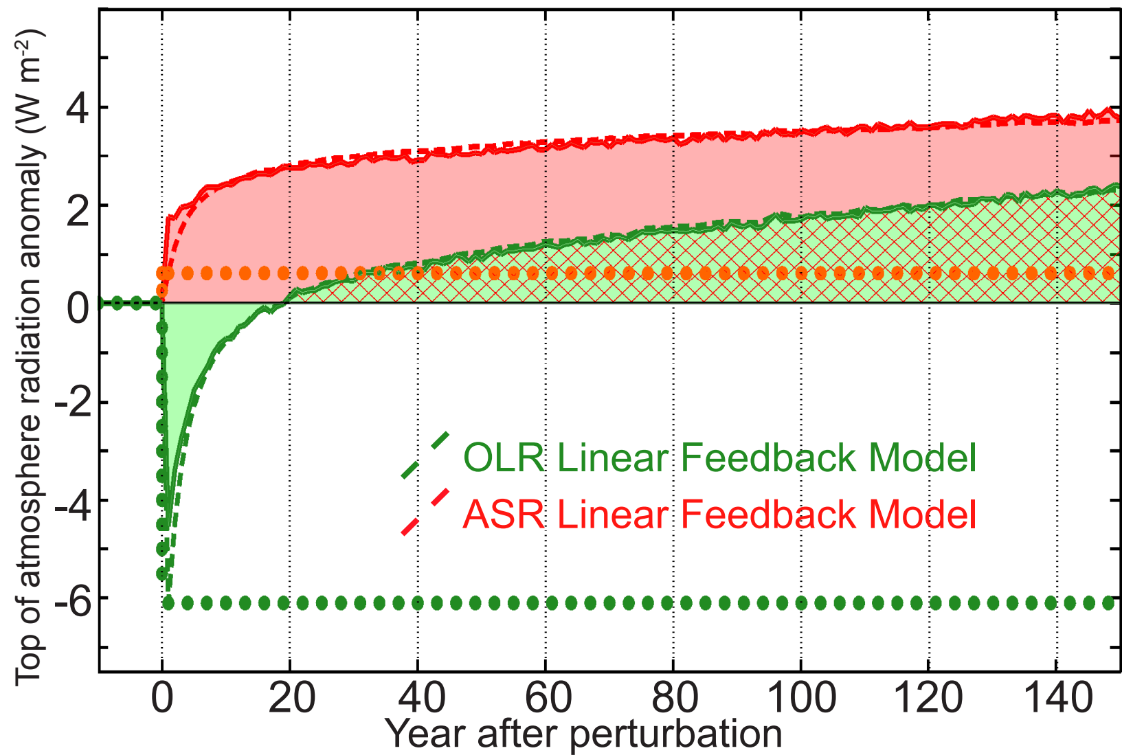
C CMIP5 Ensemble mean response instantaneous 4\times\text{CO}_2
