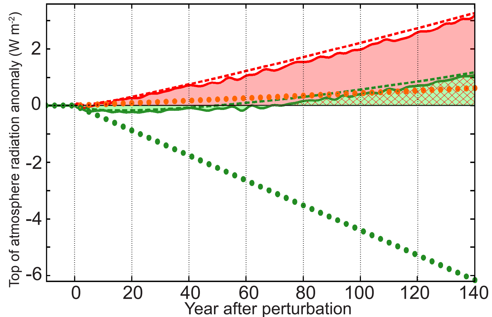
D CMIP5 Ensemble mean response to 1\%\text{CO}_2 increase
