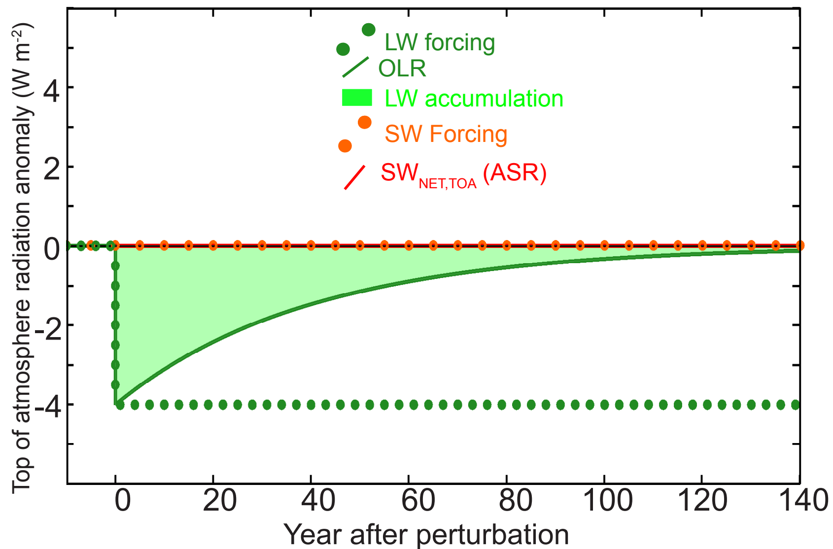
A Canonical response to instantaneous greenhouse forcing
