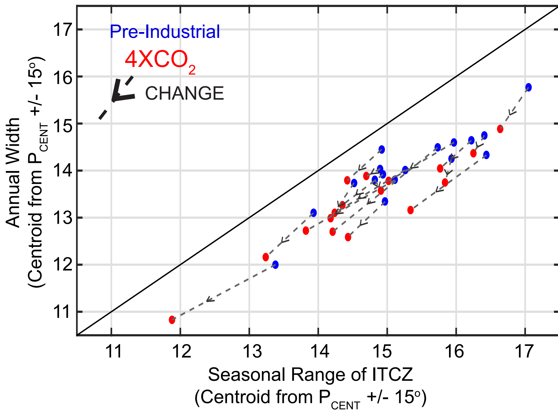
Tropical width and seasonal migration of ITCZ
