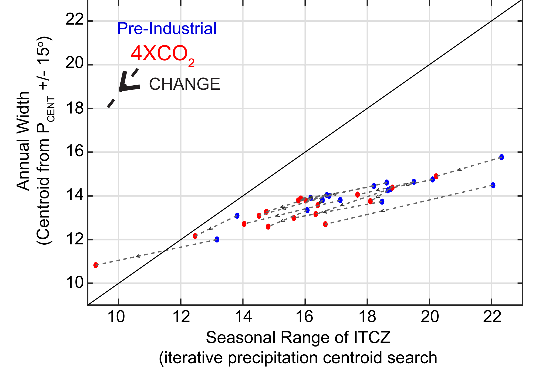
Tropical width and seasonal migration of ITCZ
