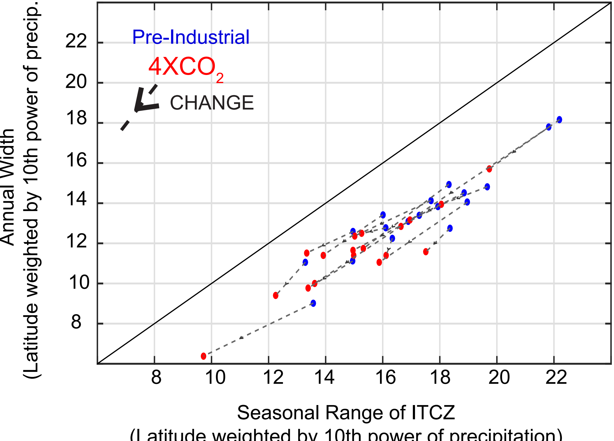
Tropical width and seasonal migration of ITCZ
